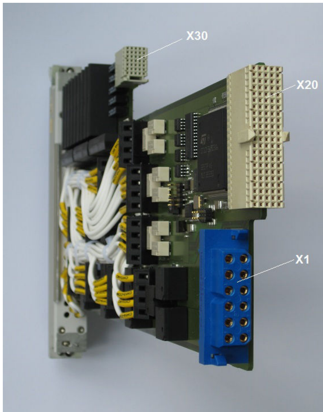
Figure 4-2: R&S TS-PSM4 Rear ( to backplane of the chassis)
