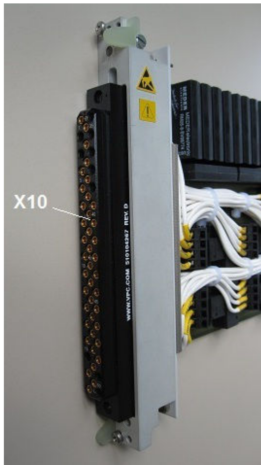
Figure 4-1: R&S TS-PSM4 (variant 03) Front with VPC
