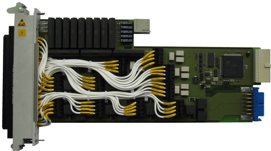
Figure 6-5: R&S TS-PSM4 (variant 03)
