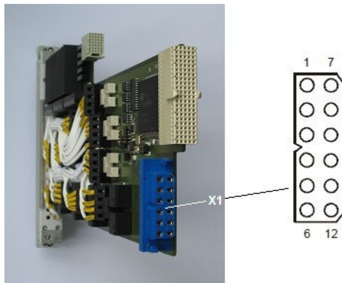
Figure 9-1: R&S TS-PSM4 connector X1 (view: plug side)
