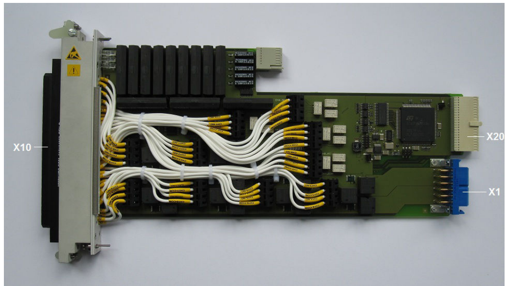
Figure 4-3: R&S TS-PSM4 (variant 03) Base board
