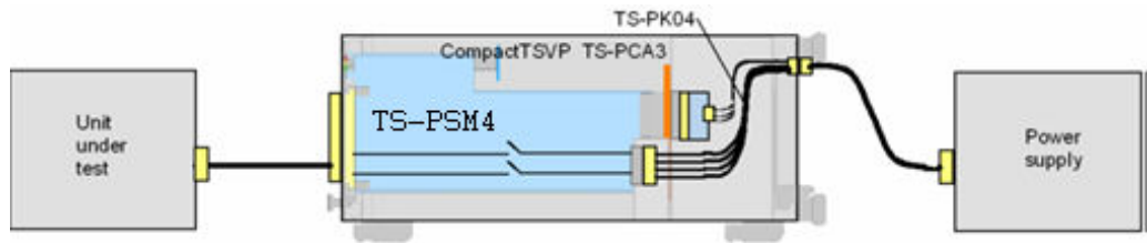
Figure 4-8: Installation of R&S TS-PSM4 with R&S TS-PK04 in the CompactTSVP R&S TS-PCA3
