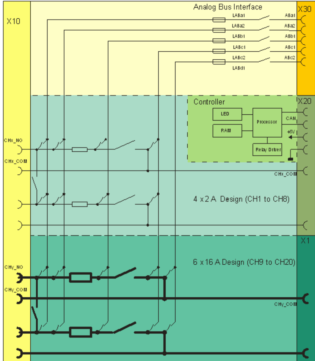
Figure 3-1: Block diagram R&S TS-PSM4
