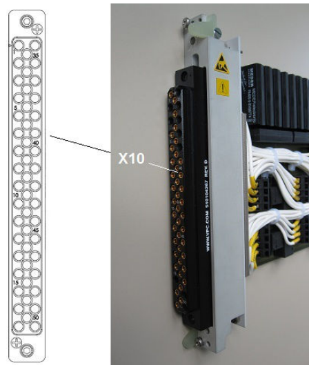
Figure 9-2: R&S TS-PSM4 (variant 03) connector X10
