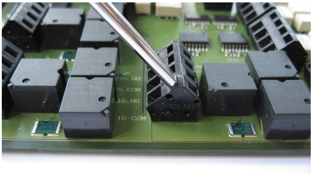
Figure 6-3: Over the upper opening of the terminal the metal spring can be pressed down
