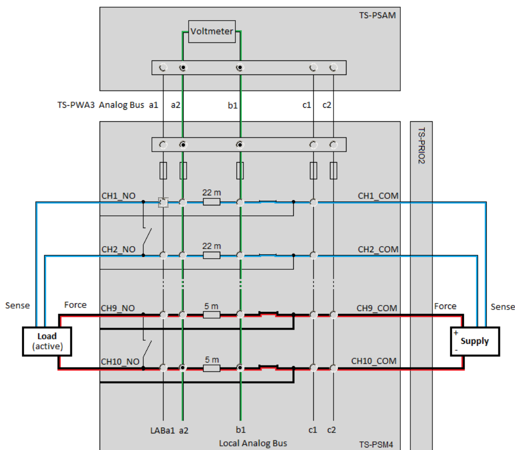
Figure 5-1: Application example - measuring current with active load
