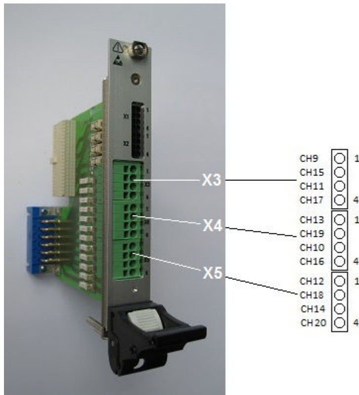
Figure 9-11: R&S TS-PRIO2 connector X3, X4 and X5
