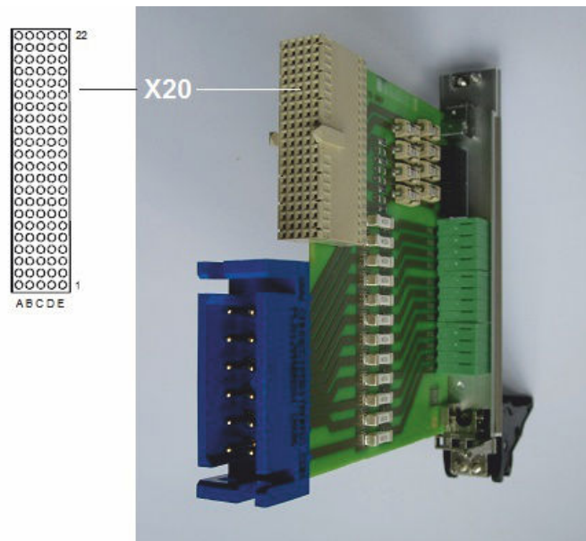
Figure 9-8: R&S TS-PRIO2 connector X20 (view: plug side)
