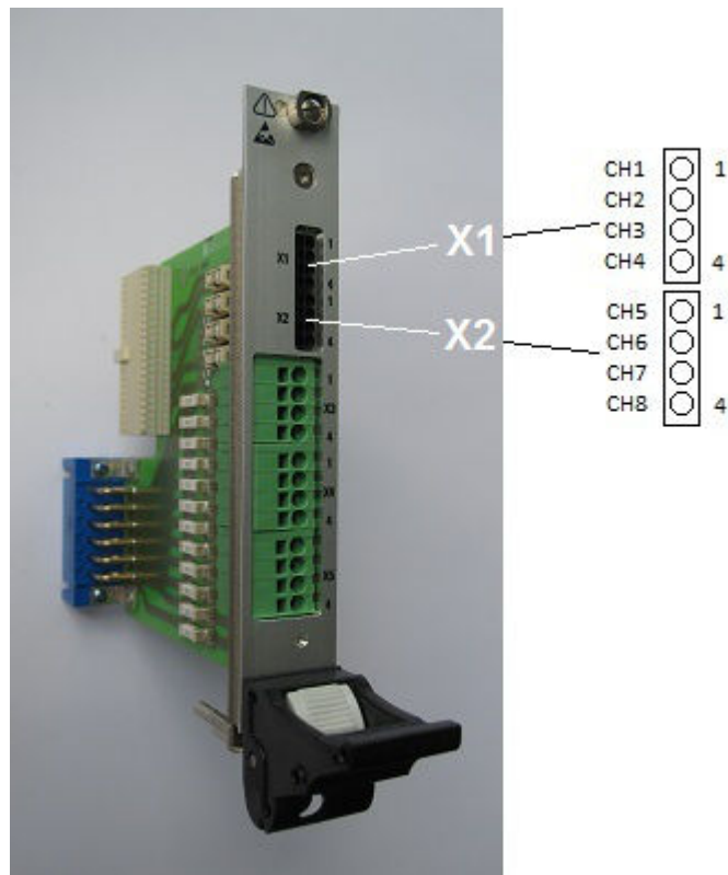
Figure 9-10: R&S TS-PRI02 connector X1 and X2
