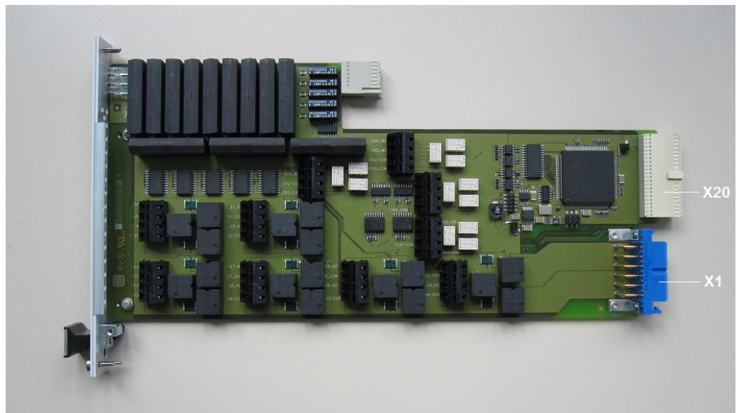
Figure 4-4: R&S TS-PSM4B (variant 02) Base board
