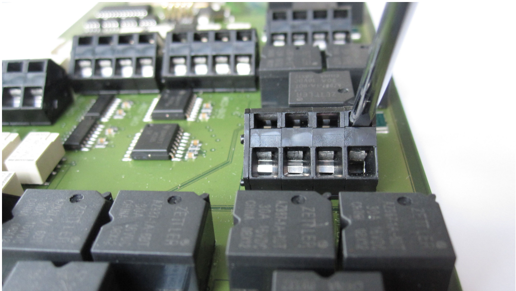
Figure 6-4: The wire can be mounted in the lower round opening
