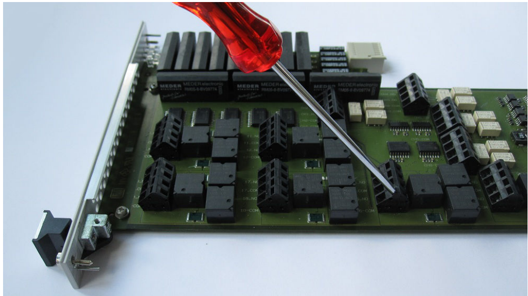
Figure 6-2: Opening the terminal contact CH16_COM
