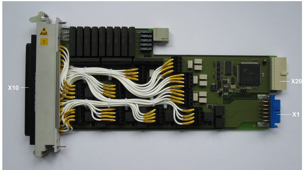
Figure 2-1: View of the R&S TS-PSM4 (variant 03)
