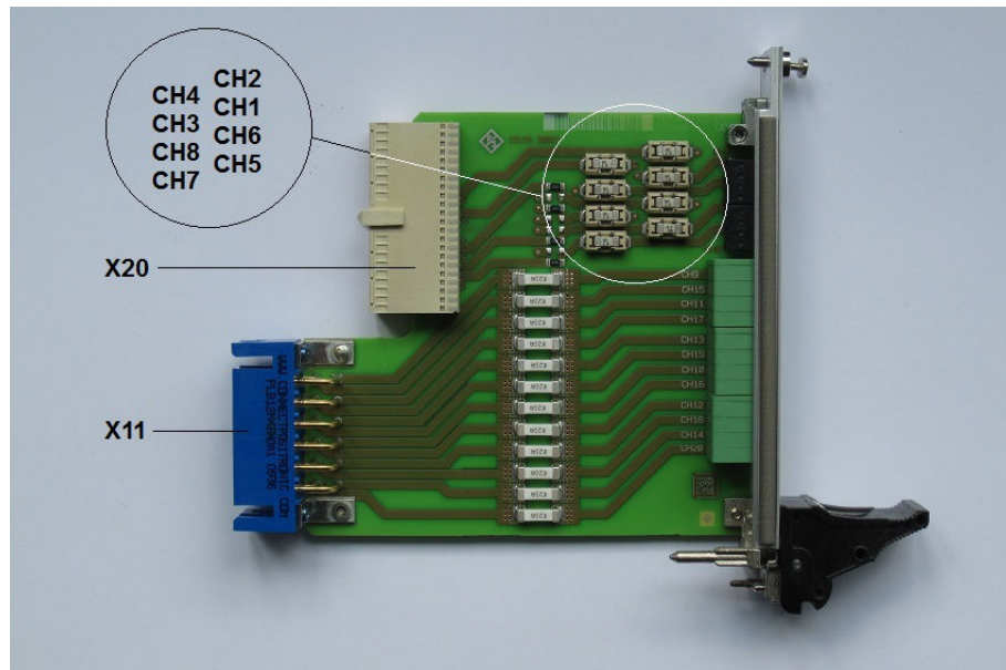
Figure 4-7: R&S TS-PRIO2 position of 3 A fuses
