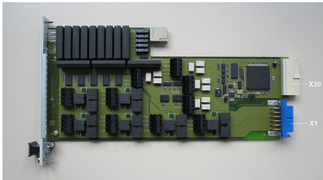
Figure 2-2: View of the R&S TS-PSM4B (variant 02)
